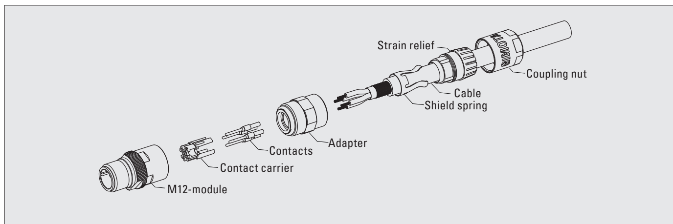
Assembly GTM12
