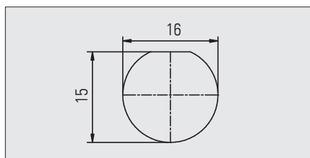
Panel cut-out
